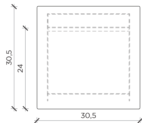
FRONTE | FRONT
